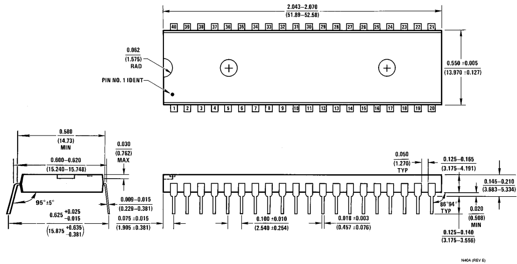
Molded Dual-In-Line Package (N) Order Number MM5483N NS Package Number N40A
