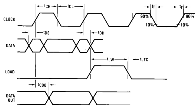
FIGURE 6. Timing Diagram
