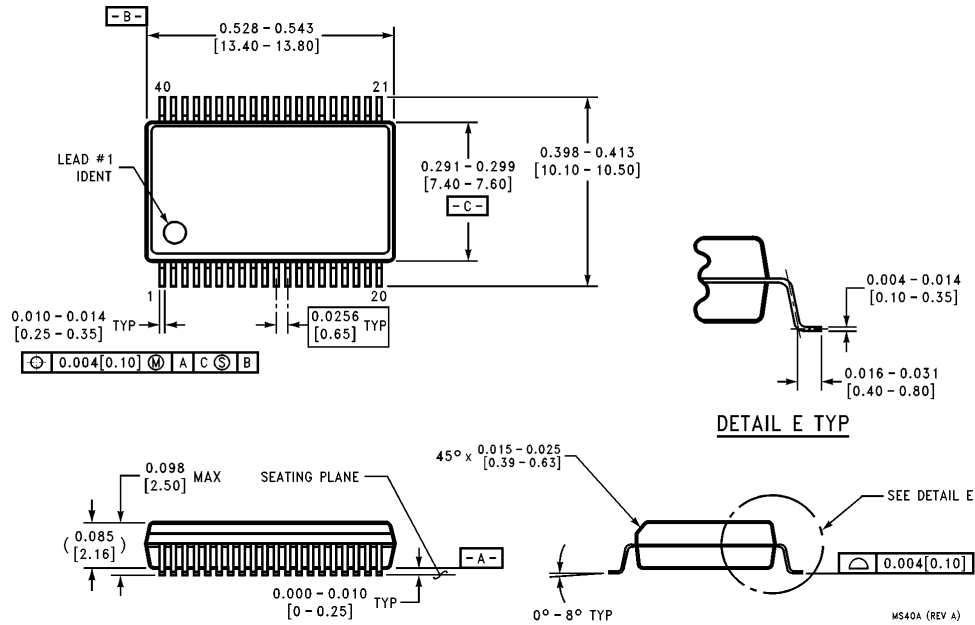
40-Lead Molded Shrink Small Outline Package, JEDEC Order Number MM5483MS NS Package Number MS40A
