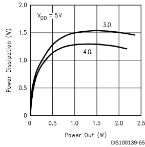
LM4835MTE Power Dissipation vs Output Power
