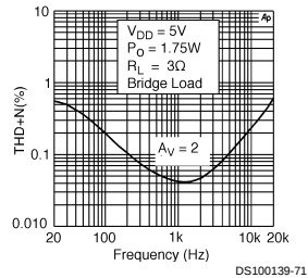
LM4835MTE THD+N vs Frequency
