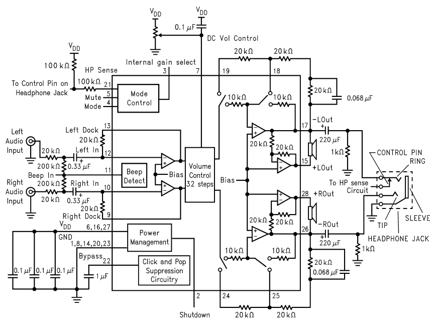
FIGURE 2. Typical Application Circuit
