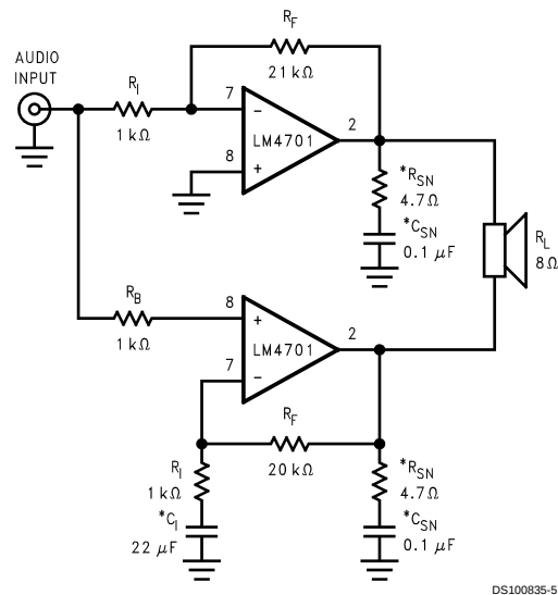
FIGURE 2. Bridged Amplifier Application Circuit
