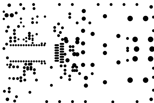
FIGURE 11. Reference PCB bottom layer solder mask
